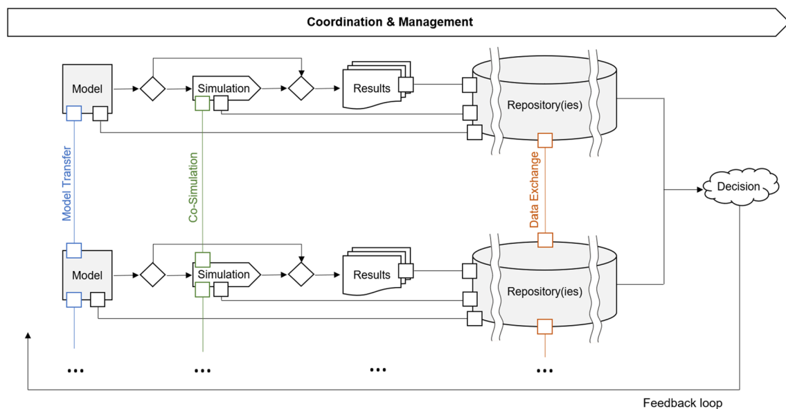
Fig. 6 Model-based development
